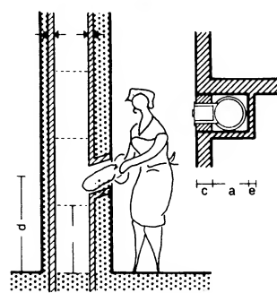
⑫ Waste disposal in bags
